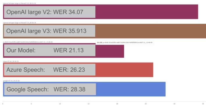
Automatic Speech Recognition WER score among commercial APIs
